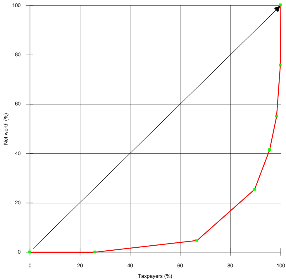
Lorenz curve
