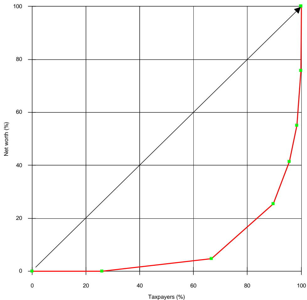
Lorenz curve
